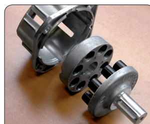
Integrated elastic joint, for best pump coupling (except model 1211).
